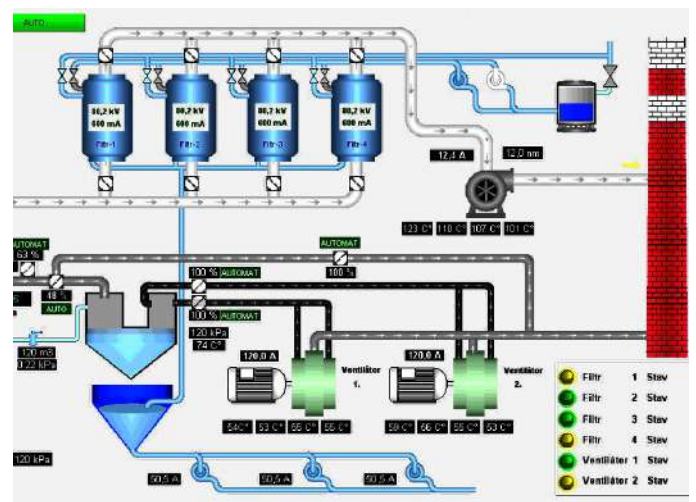
PLC Control Panel
